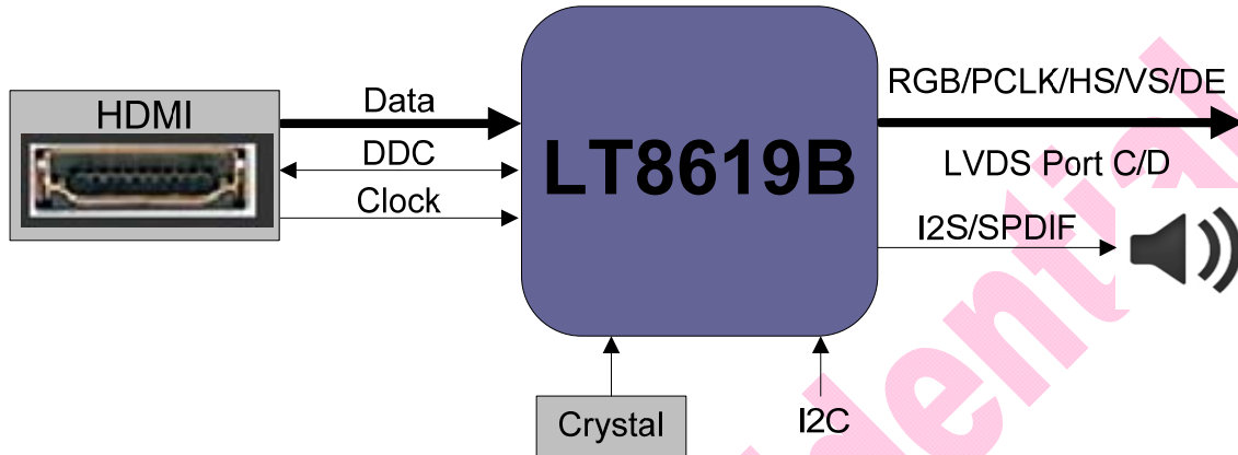
Figure 1. Application Diagram
