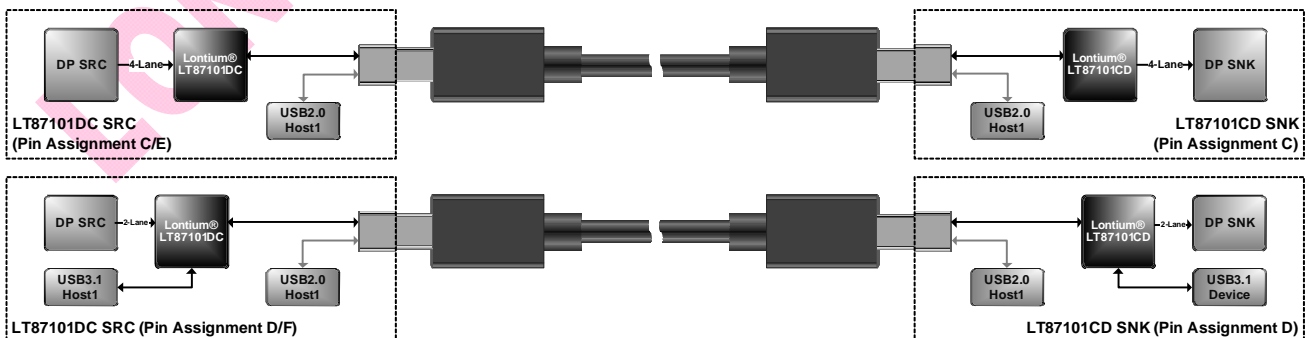
Figure 1. LT87101DC / LT87101CD Typical Application Diagram
