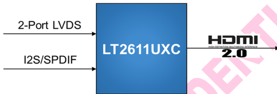
Figure1. Application Diagram
