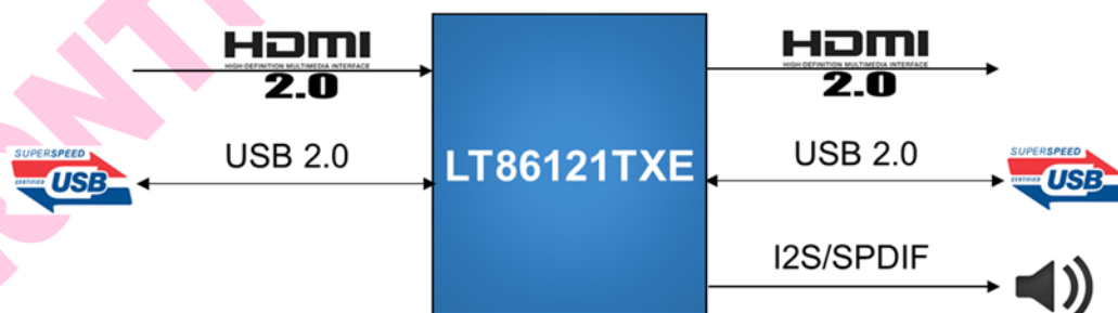
Figure1. Application Diagram
