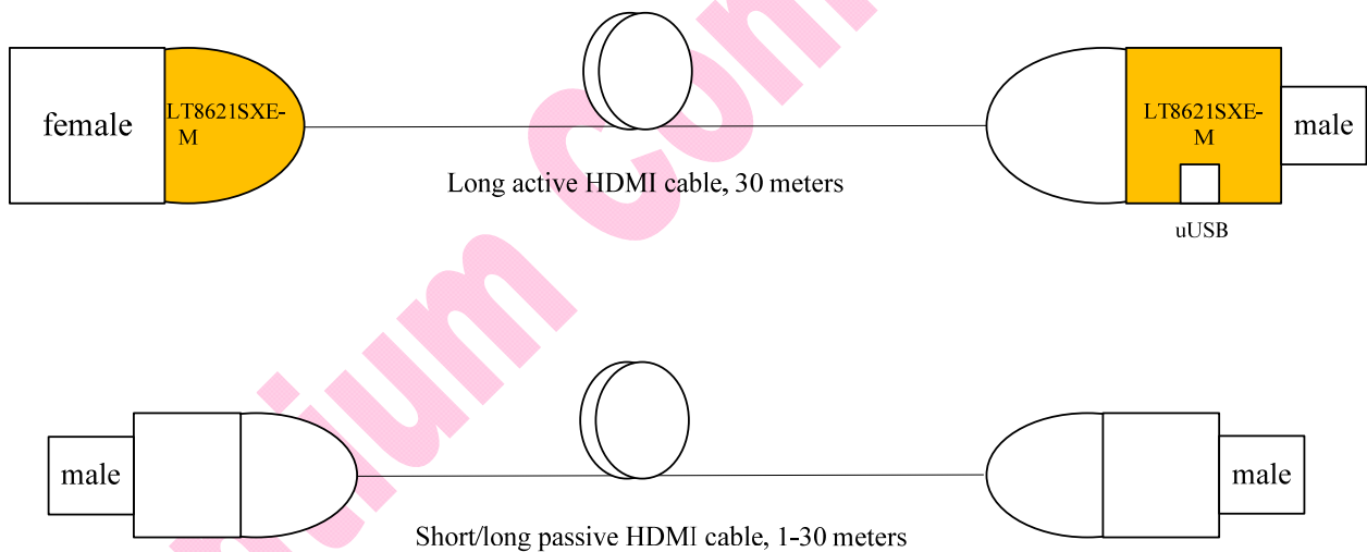
(b) HDMI Signal Extension over HDMI Cable
