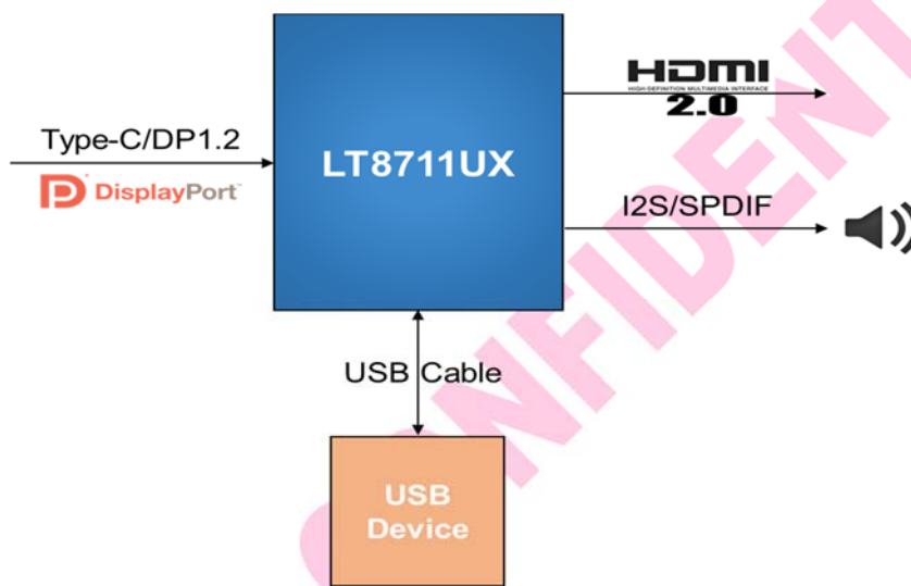
Figure 1. Application Diagram
